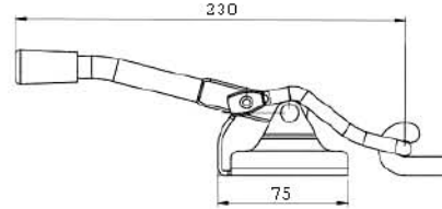
Hyundai Mekanik Kol Hyundai Mechanical Lever
