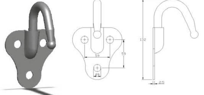
14 mm Saclı Kanca 14 mm Hook
