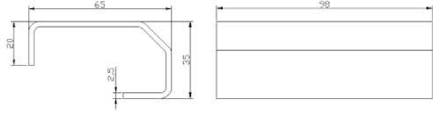
Ahşap Kasa Ayak Basamağı Foot Step for Wooden Van
