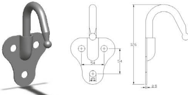
12 mm Saclı Kanca 12 mm Hook
