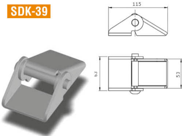
Orta Boy Damper Menteşesi (4 mm) Middle Size Dumper Hinge (4 mm)
