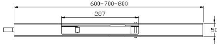
Dikey Kilitleme Sistemi Kod SDK581 Long-Range Built-in Bolt Fastener Code SDK581
