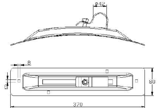
Çamurluk Kelepçesi Kod SDK1002 Tube for Mudguard Code SDK1002
