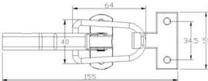
Mekanik Kol Mechanical Lever
