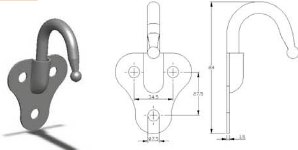
8 mm Saclı Kanca 8 mm Hook
