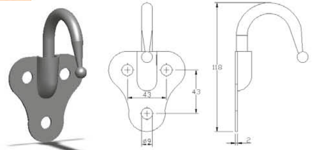
11 mm Saclı Kanca 11 mm Hook
