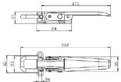
Hyundai Mekanik Kol Hyundai Mechanical Lever
